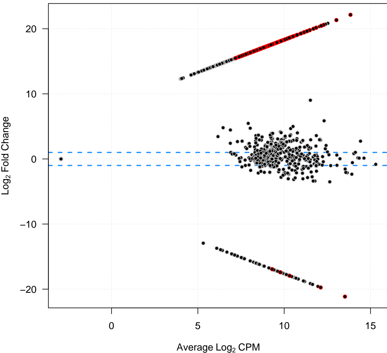
edgeR Fold Change Smear Plot
